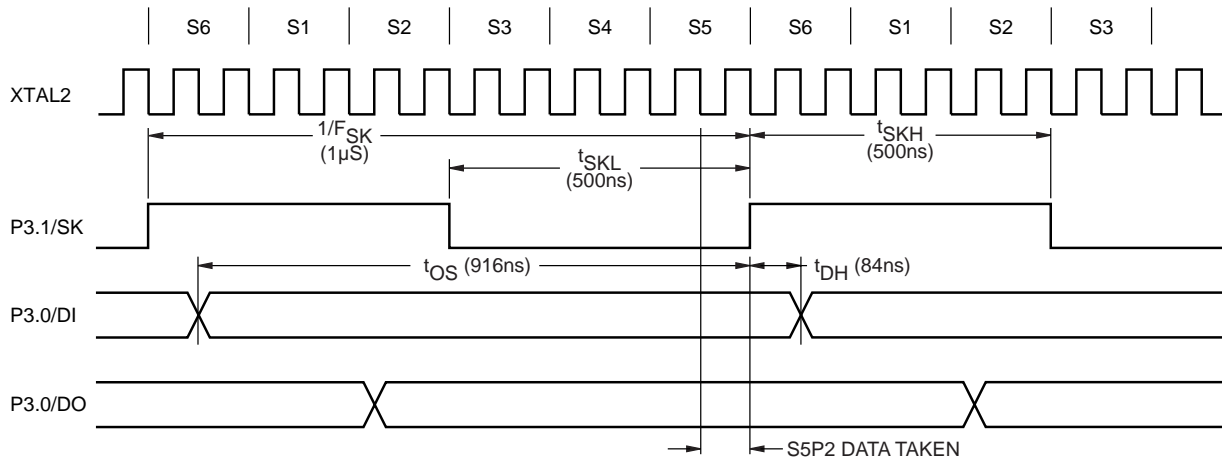
FIGURE 3. 12MHZ 8051 SERIAL PORT MODE 0 AND X24C44 TIMING
